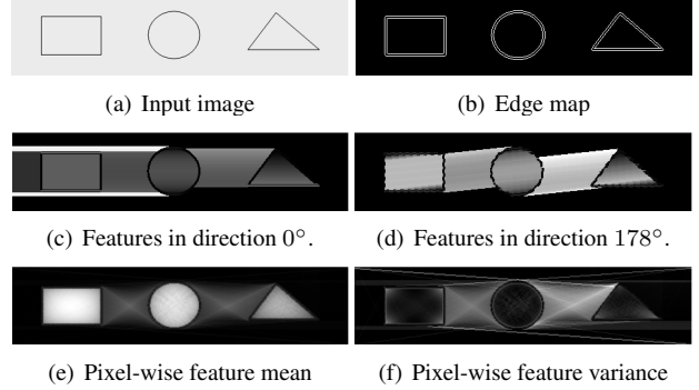
Figure 4. Illustration of Radon-Like features when used with the extraction function T_1 (Eq. 3).
