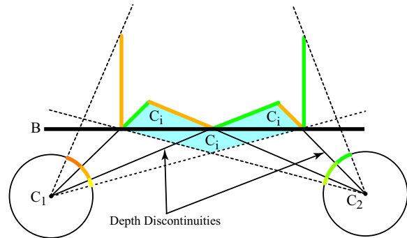
Figure 4: Segmentation along depth discontinuities allows to correctly determine consistency with fewer than four colors.
