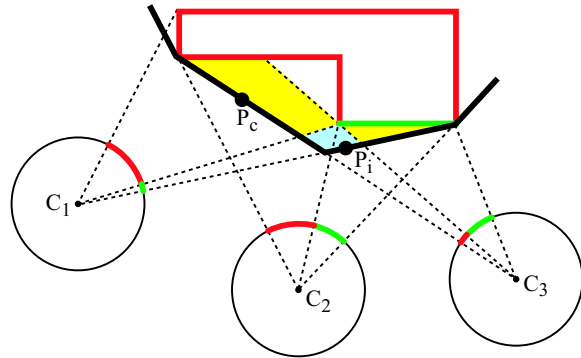
Figure 2: 2D example of consistency. P_i is inconsistent because the region IDs of its projections are not the same. P_c is consistent. Cyan cells are inconsistent, and yellow cells consistent. The thick black outline is the initial volume.
