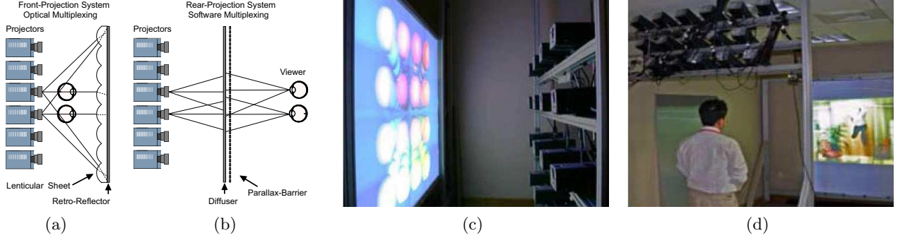
Figure 3. Rear-projection and front-projection multiview parallax displays setups are shown in 3(a) and 3(b). Equivalent systems can be built using parallax-barriers instead of lenticular sheets. 3(c) shows our front-projection lenticular display implementation with optical multiplexing and 3(d) shows our rear-projection parallax-barrier display with software multiplexing.
