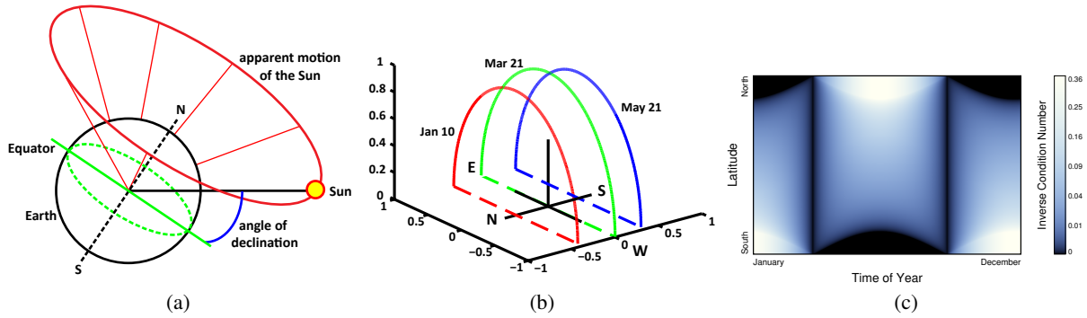
Figure 2: (a) An earth-centric illustration of the motion of the sun. The axis of the earth’s rotation is inclined at an angle of 23^{\circ}27' to the plane of its orbit around the sun. This creates an angle of declination (shown in blue in (a)) between the N-S axis and the earth-sun line. As a result, the sun moves in a great plane (shown in red) that is offset from the equatorial plane, and the sunlight rays are non-planar. As the earth revolves around the sun, the angle of declination varies from a \pm 23^{\circ}27' during the solstices to 0^{\circ} at the equinoxes. This leads to different solar planes as illustrated in (b), where we have plotted the position of sun at 0^{\circ}N , 0^{\circ}E for three different days. The planes are different and the plane on Mar. 21 (the vernal equinox) passes through the origin, making all sunlight directions co-planar. While the sunlight directions are non-planar during all other times of the year, the stability of the photometric stereo problem depends on the conditioning of the sunlight matrix. This is illustrated in (c), that shows a visualization of the inverse of the condition number (ratio of minimum to maximum eigenvalues) of the light direction matrix, for varying latitude and date. The matrix is singular in the polar regions during winter (since the sun is not visible) and worldwide on the vernal and autumnal equinoxes (since the path of the sun is planar on those dates). Otherwise, the matrix is nonsingular, indicating that normal estimation is possible.
