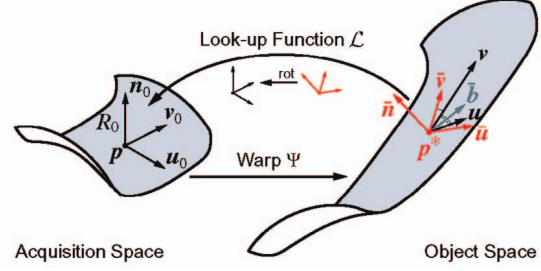
Fig. 7. For each point on the impostor geometry, the local impostor parameterization provides two coordinate systems: The orthogonal tangential system R_0 in p_0 in the acquisition frame and its warped counterpart on the rendered impostor geometry in object space, defined by p^* and (u, v) . During rendering, p_0 , R_0 , and the orthogonalized tangential system (\bar{u}, \bar{v}) are used to determine the appearance-preserving back-projection of the SRF query.
