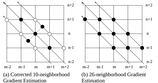
Figure 6: Gradient Estimation Schemes.
