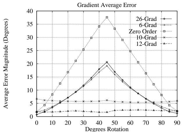
Figure 2: Average error magnitude of comparing different ABC gradient estimation schemes to the true analytic normal on a voxelized sphere.
