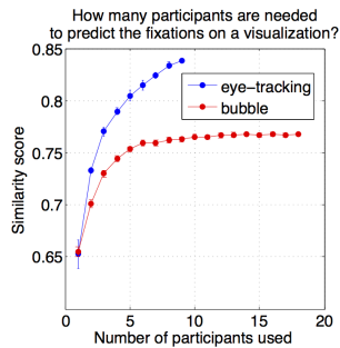
Figure 5: When there is little or no human eye-tracking data available, bubble clicks can help predict ground-truth fixations on visualizations (as compared to a chance baseline with a similarity score of 0.33, see text). However, we also observe systematic differences between the two modalities.
