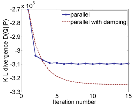
Figure 5. Damping helps convergence. The parallel mean field algorithm (blue circle) fails to converge for the fully connected layered model, while damping (red dot) helps the algorithm to converge to a better local minimum.
