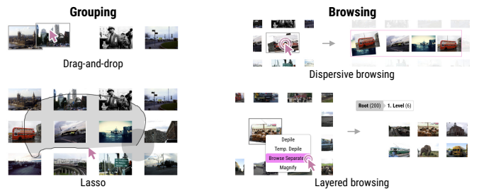
Fig. 9. Interaction Techniques. PILING.JS supports drag-and-drop and lasso gestures for manual grouping. In PILING.JS, piles can be dispersed temporarily via a double click and browsed in layers via the context menu.
