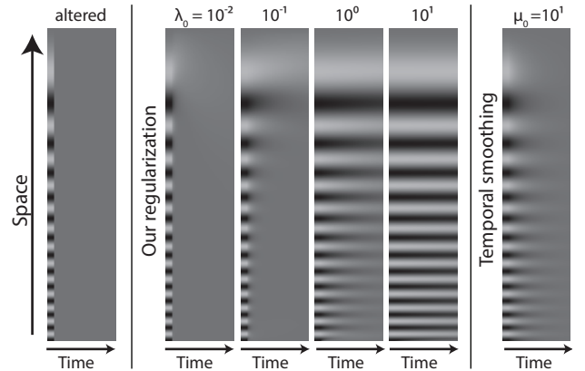
Figure 2: We perform a synthetic experiment on a 1D video: each frame is a vertical line of pixels. The first frames show a linear chirp, i.e., a signal of increasing spatial frequency, and the remaining frames are uniformly gray. With a low \lambda_0 value, there is no temporal consistency and the output video transitions instantly back to a uniform color. For intermediate values, the temporal consistency is enforced more strongly on the low frequencies which remain visible for a long time, while the high-frequency region at the bottom is allowed to be temporally discontinuous and quickly becomes uniform. For a large \lambda_0 value, temporal consistency is enforced on the whole spectrum and the chirp is propagated to all frames. These results are predicted by our analysis (§ 3.2). Right: In contrast, temporal smoothing enforces consistency uniformly over the spectrum.
