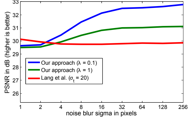
Figure 3: We analyze our algorithm behavior on a synthetic reflectance-only video by adding a random per-frame offset and noise filtered by a Gaussian filter with increasing standard deviation. The PSNR of the deteriorated reflectance is kept constant at 25.3dB across noise scales. At the finest scale of noise, our temporally coherent reconstruction improves the PSNR by 4.3dB to 29.6dB. The temporal smoothing algorithm of Lang et al. performs better (30.1dB). As the scale of the filter increases beyond 4 pixels, this trend changes and our approach performs better with a difference that reaches +4dB for 32 pixels and higher.
