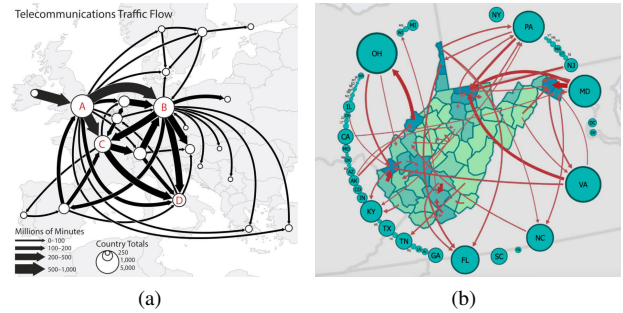
Figure 14: Examples for COMP –Superimposed: (a) A flow map using curved arrows [JSM*18] (reprinted by permission of the publisher, Taylor & Francis Ltd, www.tandfonline.com ), (b) Nodes laid out around a map [SJ17].
